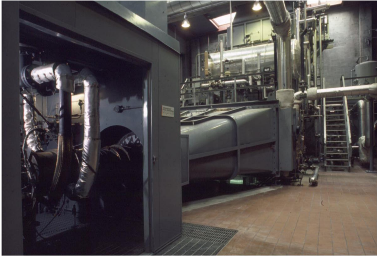
San Jose State University 6MW Cogeneration Plant Allison 501-KH (Cheng Cycle) gas turbine w/steam injection Built and developed by IPT in 1985 - currently operational Over 147,000 hours of operation - Tours available on request
