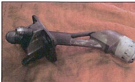
Dual Fuel Nozzle. Stock dual fuel nozzle designed to operate on natural gas and distillate. Nozzle tip has twelve 0.100-inch diameter holes.
