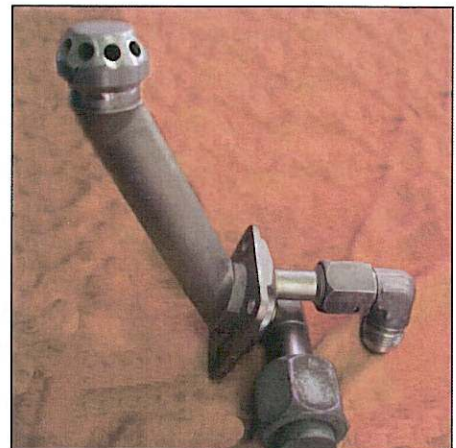
Low-Btu Nozzle. Stock steam injection nozzle designed for conventional NOx reduction and natural gas fuel injection, with ten 0.210-inch diameter holes.
